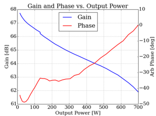
Figure 4: Gain and phase vs. output power.
