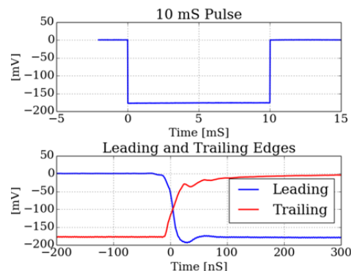
Figure 6: Pulse mode detected RF output.
