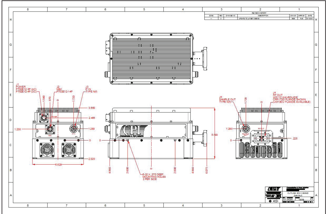
SB47XOA Series Outline Drawing 12039, rev 3, dated 13 December 2017.
